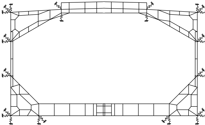
FIGURE 5 Spring Supports at Fore End of Bulk Carrier Global Models
