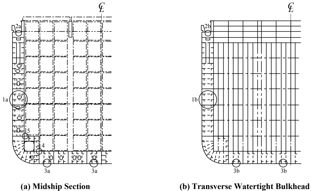
FIGURE 3 Critical Areas for Typical Containerships, Transverse Sections
