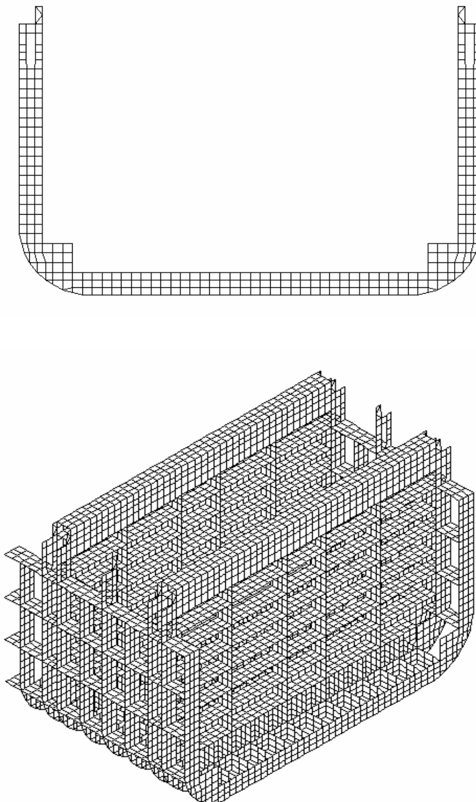
FIGURE 8 Typical Mesh Arrangement of Container Carriers
