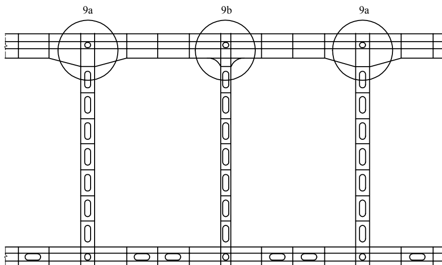
(b) Hatch-side Longitudinal Girder
