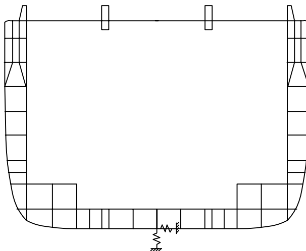
FIGURE 6 Spring Supports at Aft End for Container Carrier Global Models
