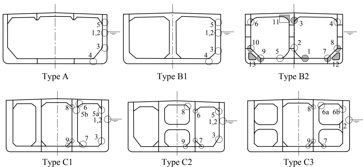
FIGURE 1 Critical Areas – Tankers
