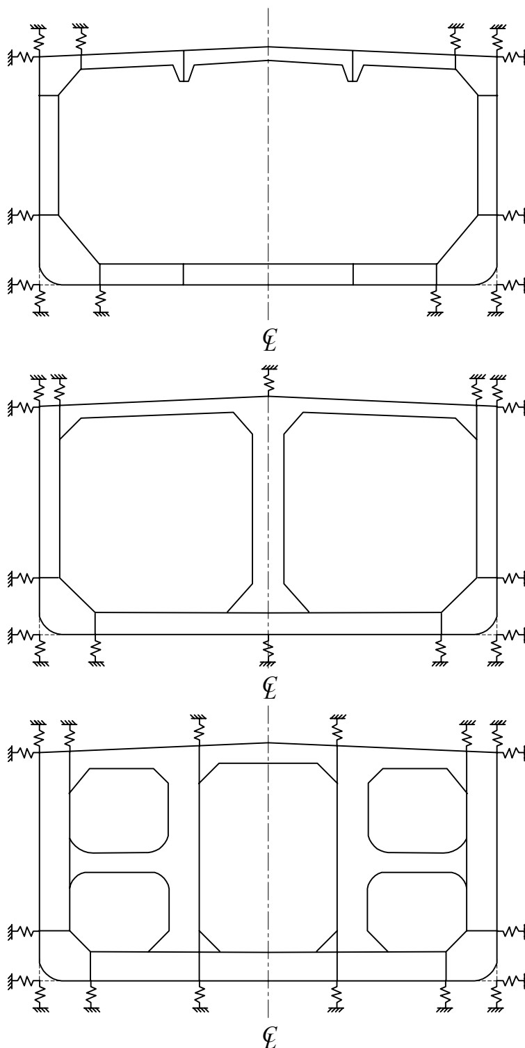
FIGURE 4 Spring Supports for Tanker Global Models
