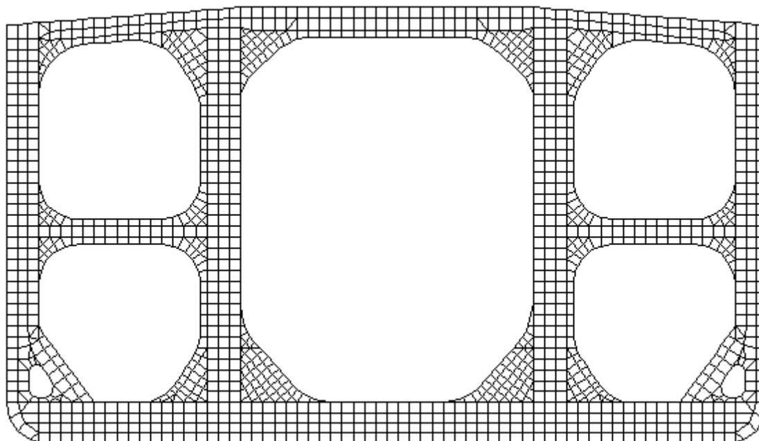
FIGURE 6 Typical Mesh Arrangement of VLCC Oil Tankers
