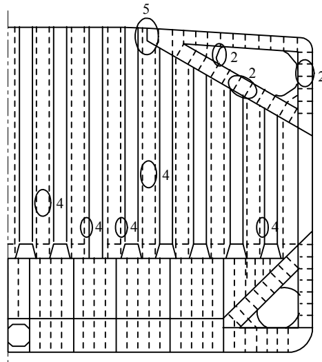
(c) Typical Transverse Bulkhead Section (without upper stool)
