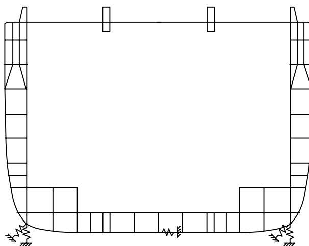
FIGURE 7 Spring Supports at Fore End for Container Carrier Global Models
