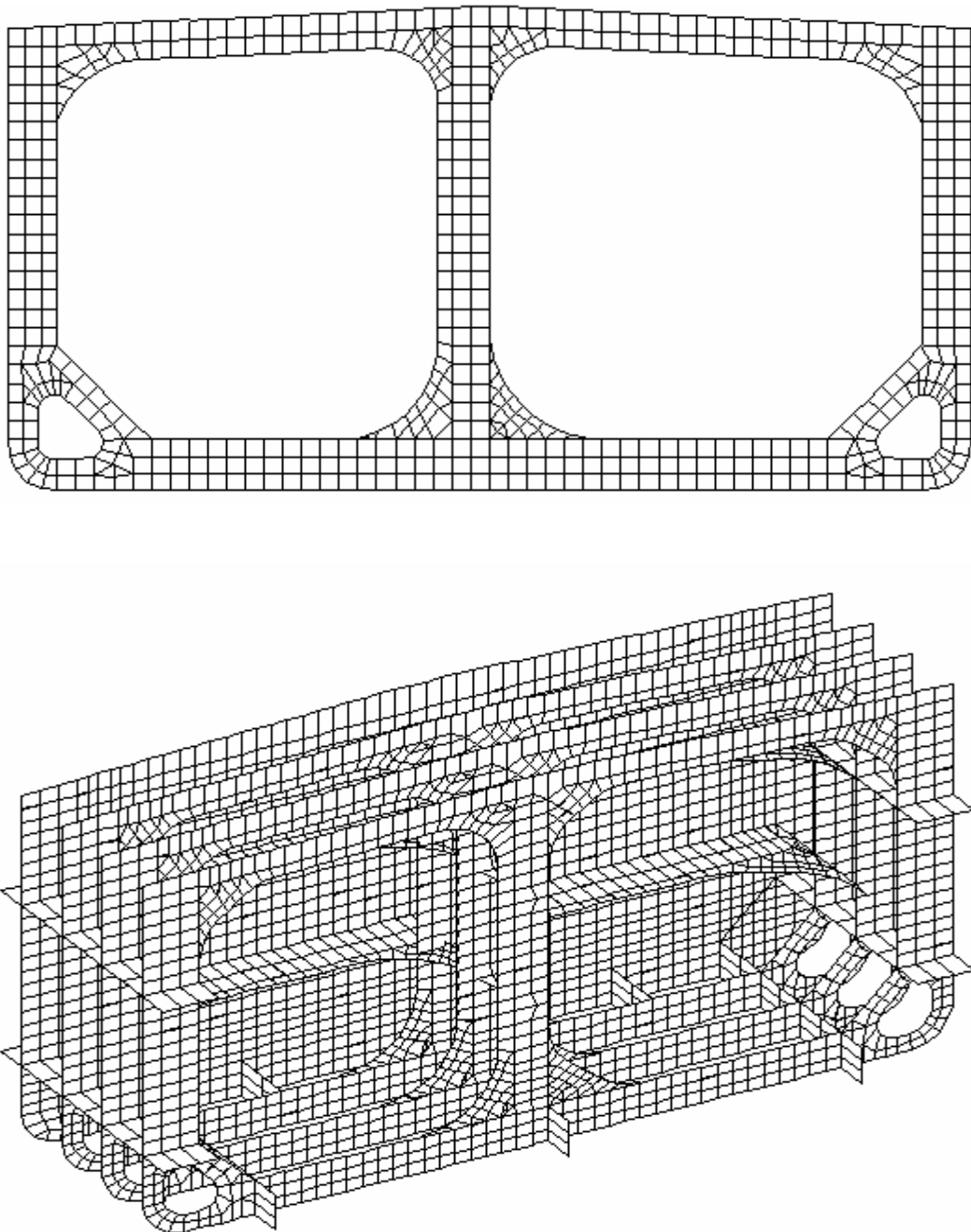
FIGURE 5 Typical Mesh Arrangement of Aframax Oil Tankers
