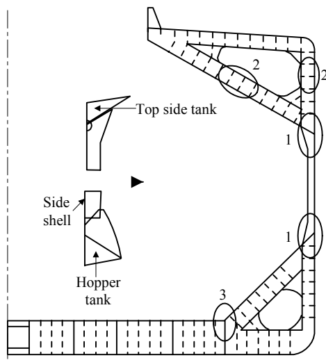
(a) Typical Midship Section
