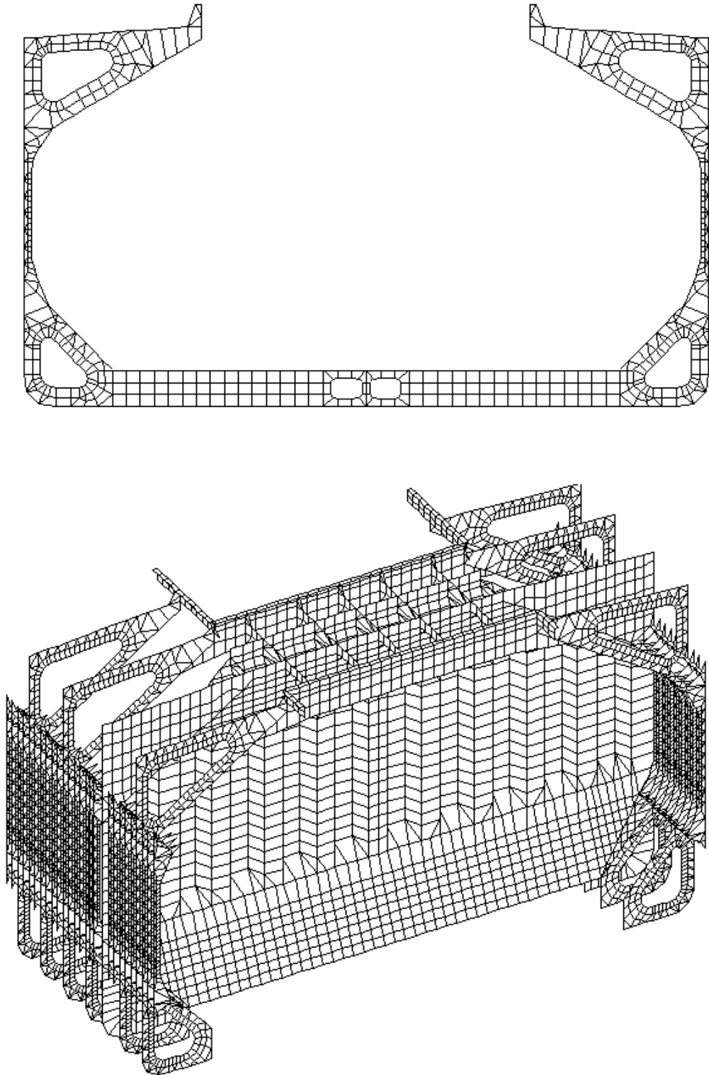
FIGURE 7 Typical Mesh Arrangement of Cape Size Bulk Carriers
